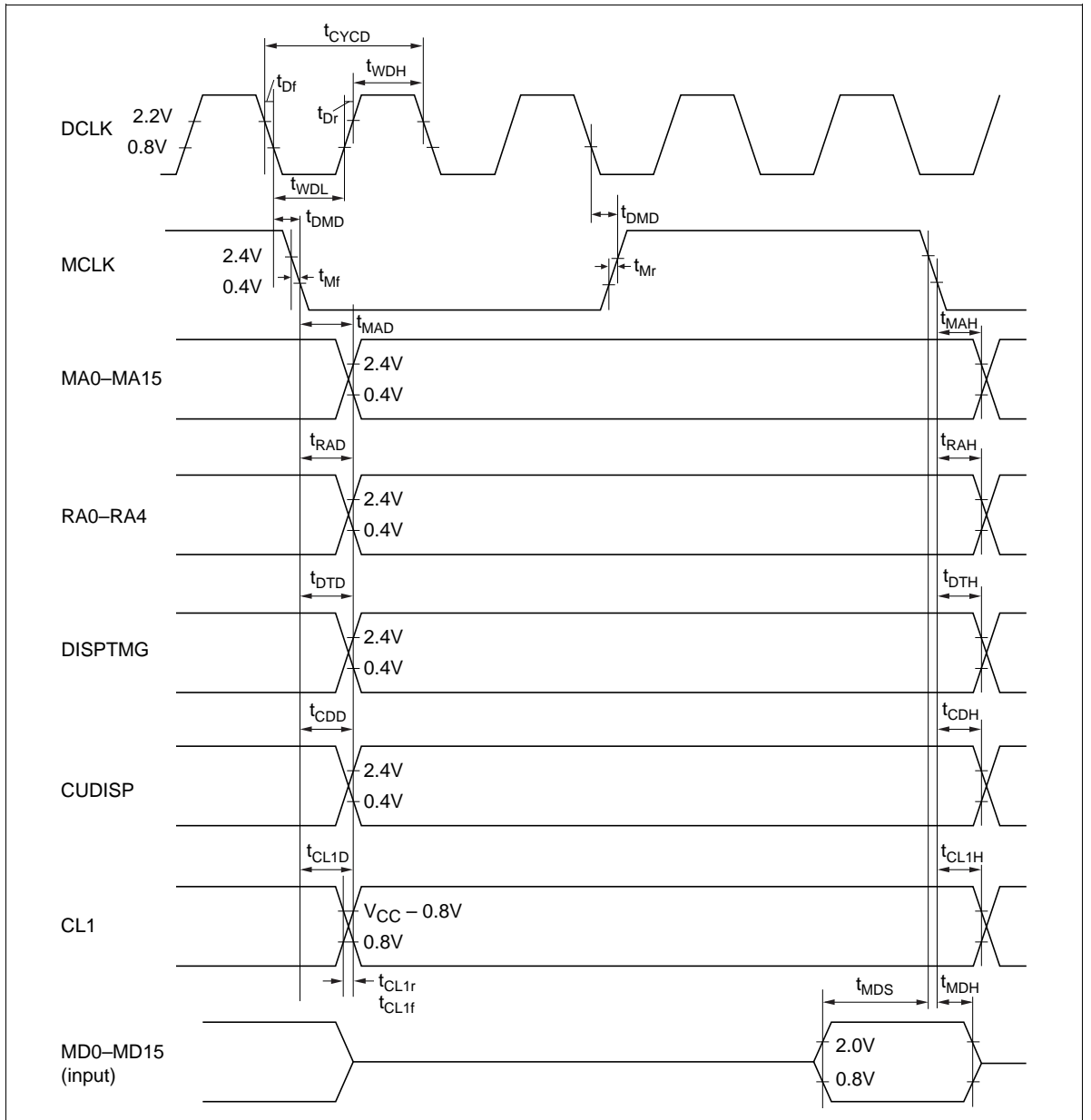
Figure 37 Memory Interface
